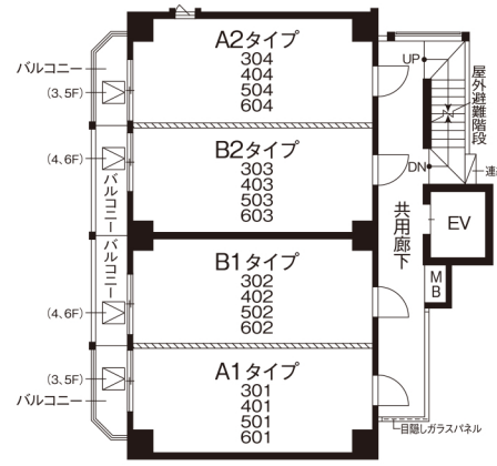
3th-6th.floor
