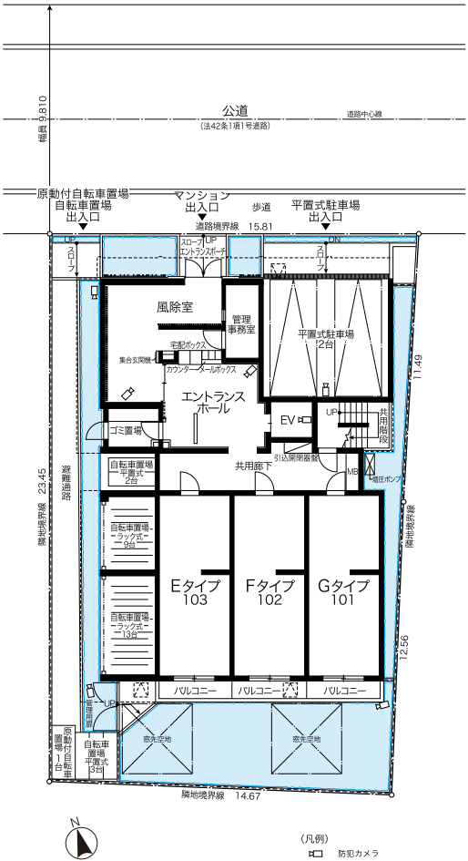
1st.floor
