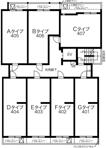
4th.floor
