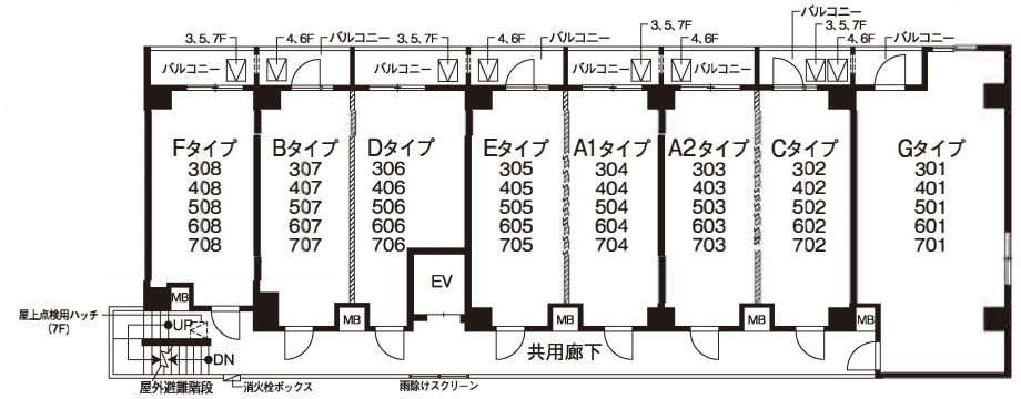
[3F~7F平面図] SCALE:約1/250
