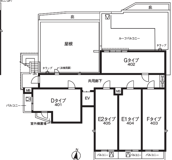
4th FLOOR
