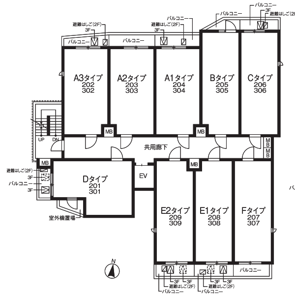
2nd-3rd FLOOR
